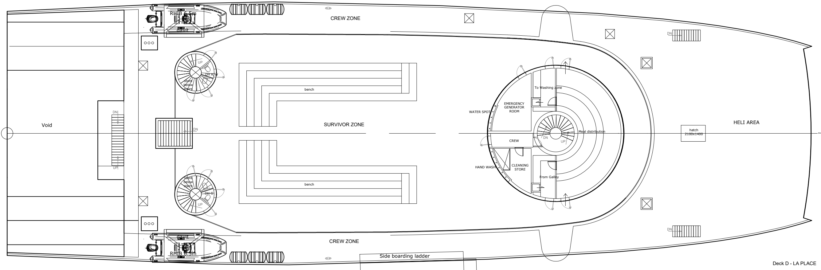
Deck D - LA PLACE
