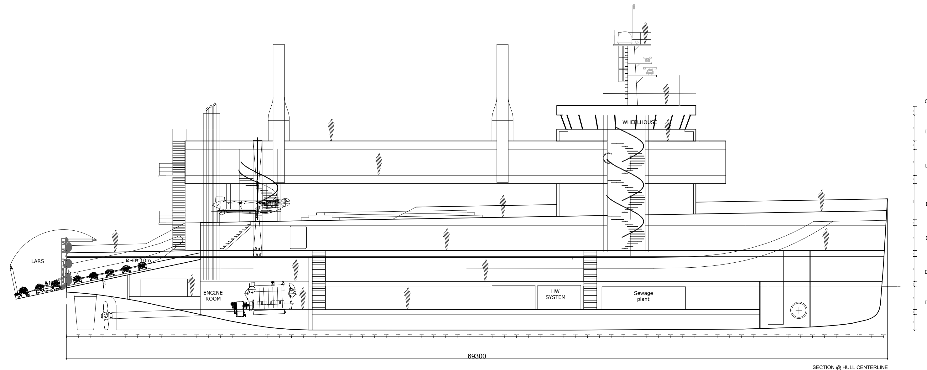
SECTION G - HULL CENTERLINE
